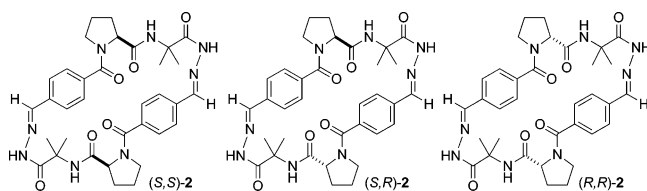
Chart 1. Diastereomers of 2
